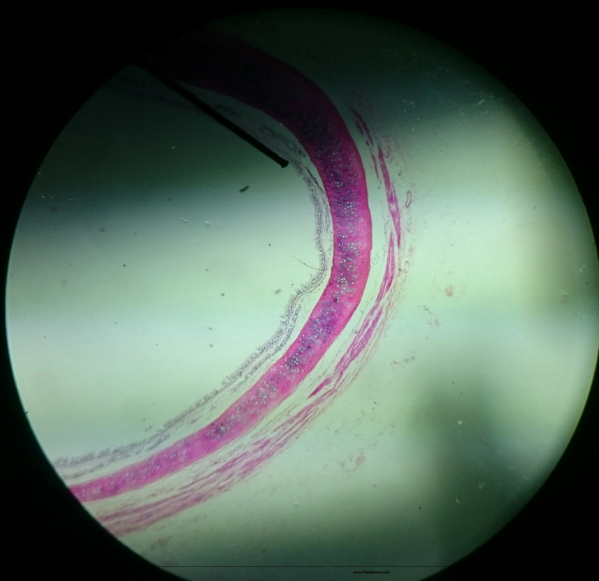
trachea 10x
