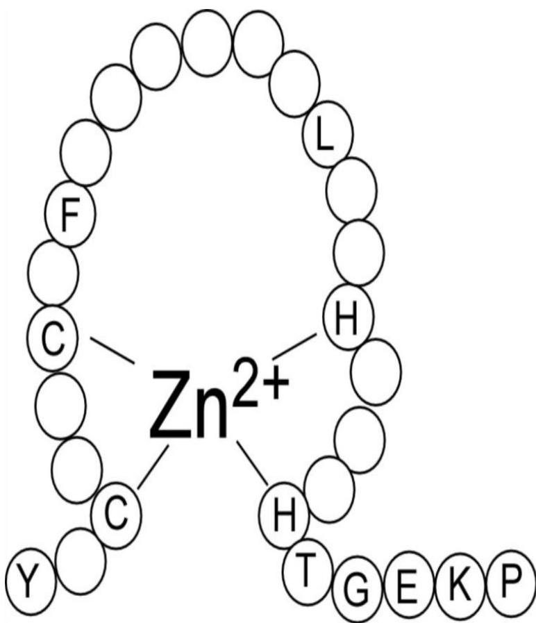
Structure of C2H2 zinc finger (C, cysteine; H, histidine)
