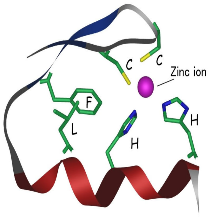
Structure of C2H2 zinc finger (C, cysteine; H, histidine)
