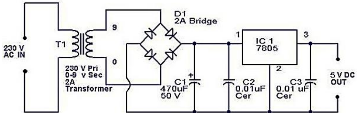
Circuit Diagram:
