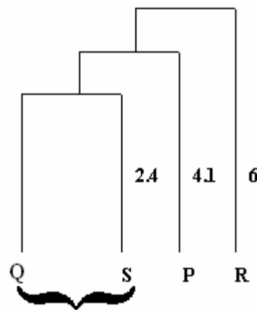
Dendrogram
