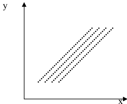
Positive Correlation
