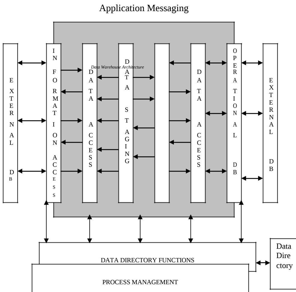
Data Warehouse Architecture
