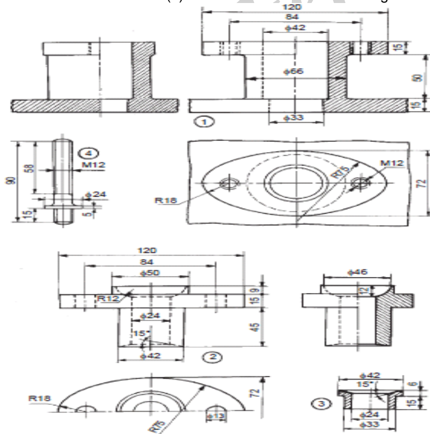
Parts list
