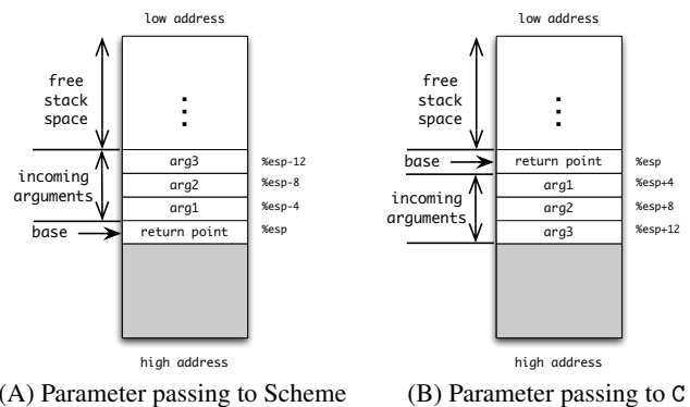
(A) Parameter passing to Scheme
