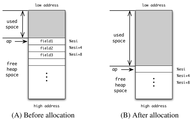
Figure 1. Illustration of the heap. The allocation pointer (ap) is held in the %esi register and its value is always aligned on 8-byte boundaries. Individual objects are allocated at address %esi and the allocation pointer is bumped to the first boundary after the object.
