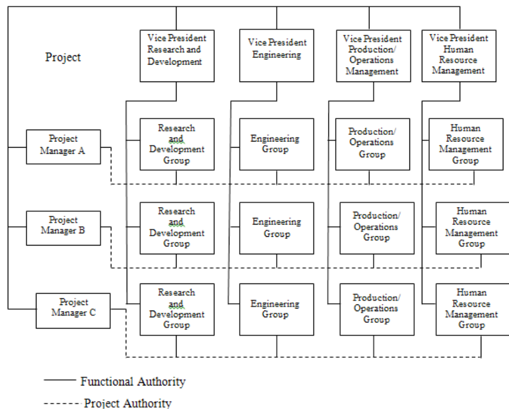
Figure 2.9: Matrix Structure
