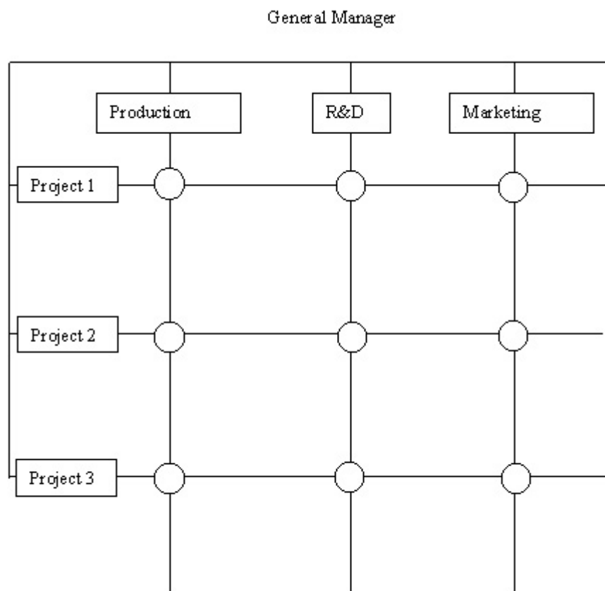
Matrix Structure
